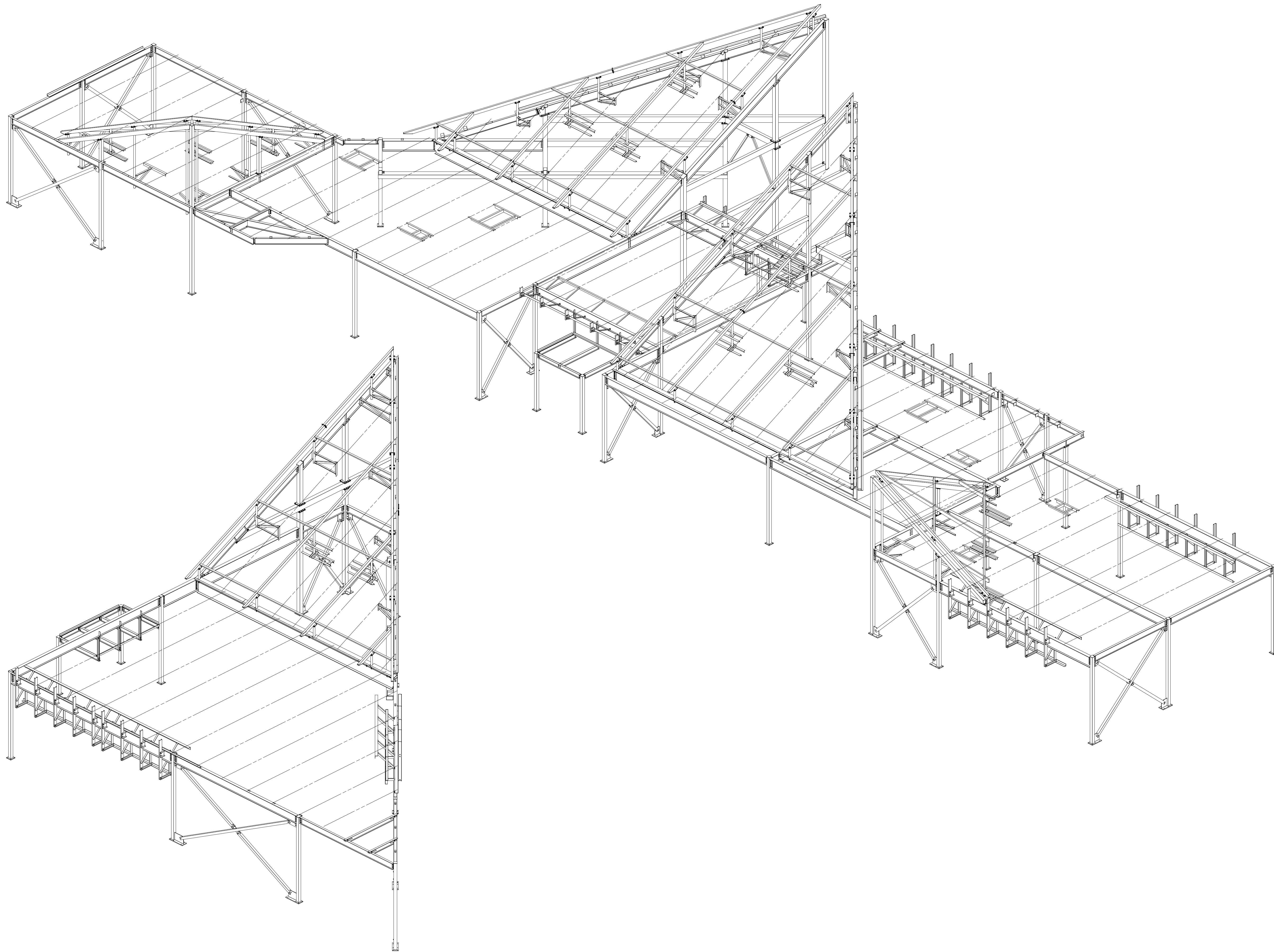
DALLAS EXECUTIVE AIRPORT PICTORIAL VIEW LOOKING SOUTHWEST - ADMINISTRATION BUILDING AND CONFERENCE CENTER
